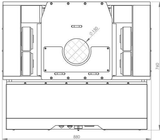
JLA-e 5/12 G | Bestell-Nr. 22 055 140-EU/USA | Draufsicht JLA-e 5/12 G | Order No. 22 055 140-EU/USA | Top view
