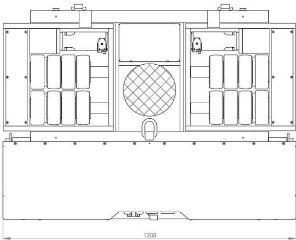
JLA-e 15/30 G | Bestell-Nr. 22 155 140-V | Draufsicht JLA-e 15/30 G | Order No. 22 155 140-V | Top view
