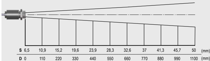
Optik CSmicro 3ML CF, D:S = 22:1 (Fernfeld 9:1)
