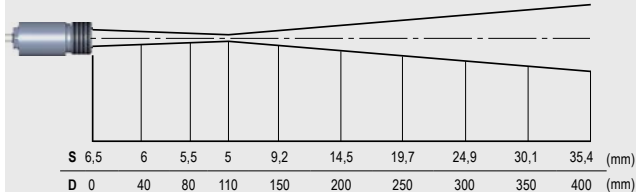
Optik CSmicro 3ML CF, D:S = 22:1 (Fernfeld 9:1)
