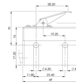
Type 4AL: Simple Lever with Roller - Direct Action -
