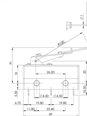
Type 7AF/63.5/50 : Simple Lever with Floater - Direct Action -
