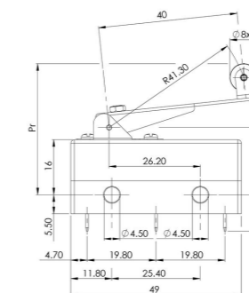
Type 8AL40 : Simple Adjustable Lever with Roller - Direct Action -
