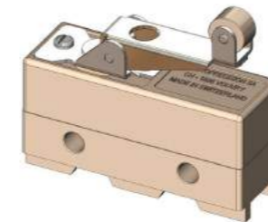
Type 6AL: Simple Lever with Bending Roller - Indirect Action -
