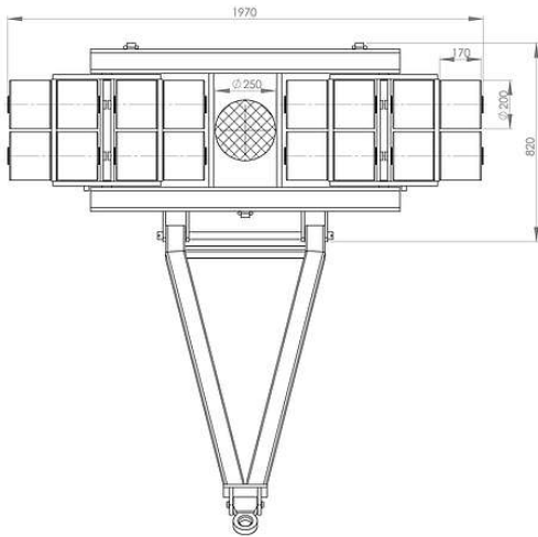
JL 80 H | Bestell-Nr. 09 800 200-H | Draufsicht JL 80 H | Order No. 09 800 200-H | Top view
